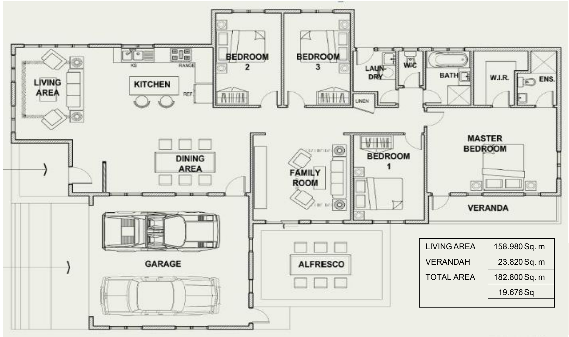
HOUSE DESIGN-BALLARAT
