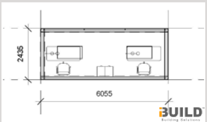
FLOOR PLAN
